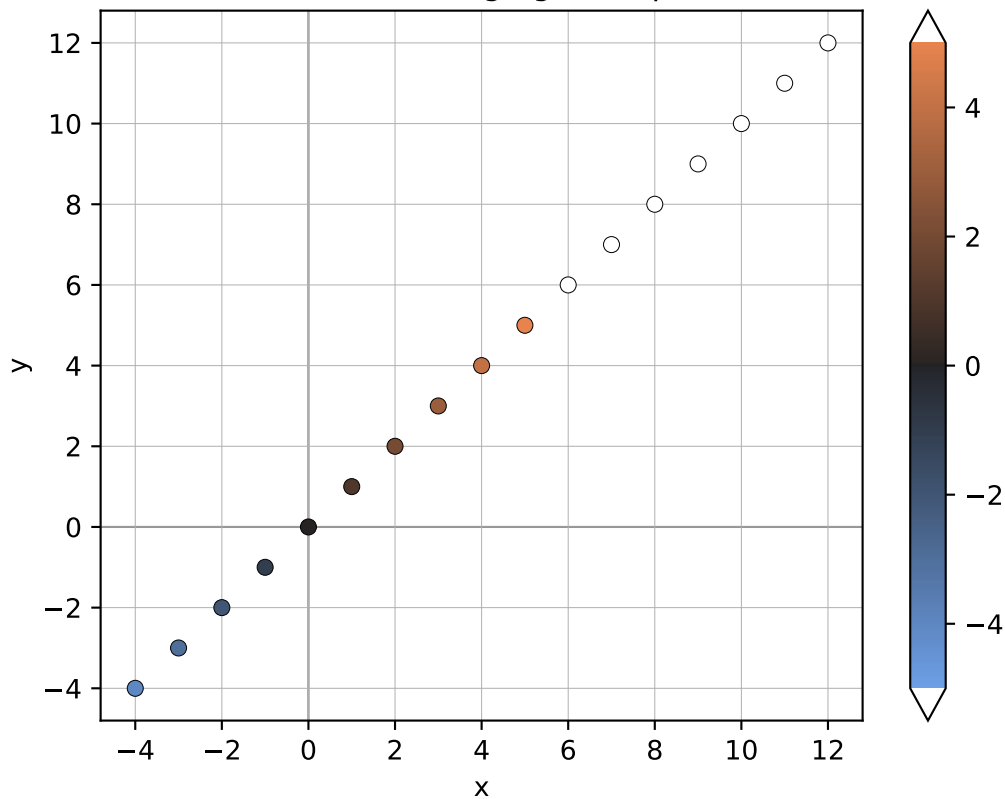
seaborn diverging example
