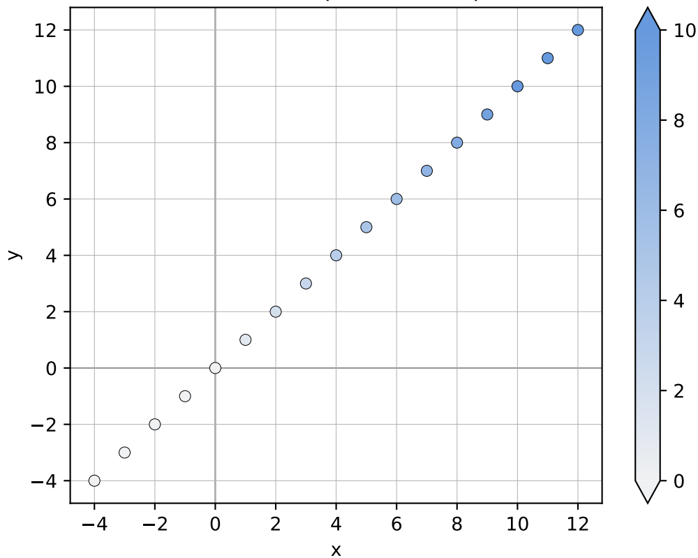
seaborn color palette example
