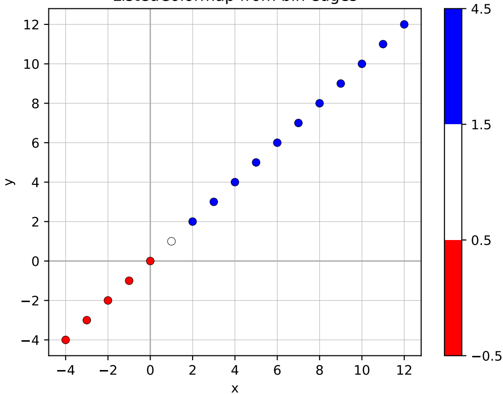
ListedColormap from bin edges
